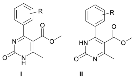
Scheme 7 Two tautomers of pyrimidines.
