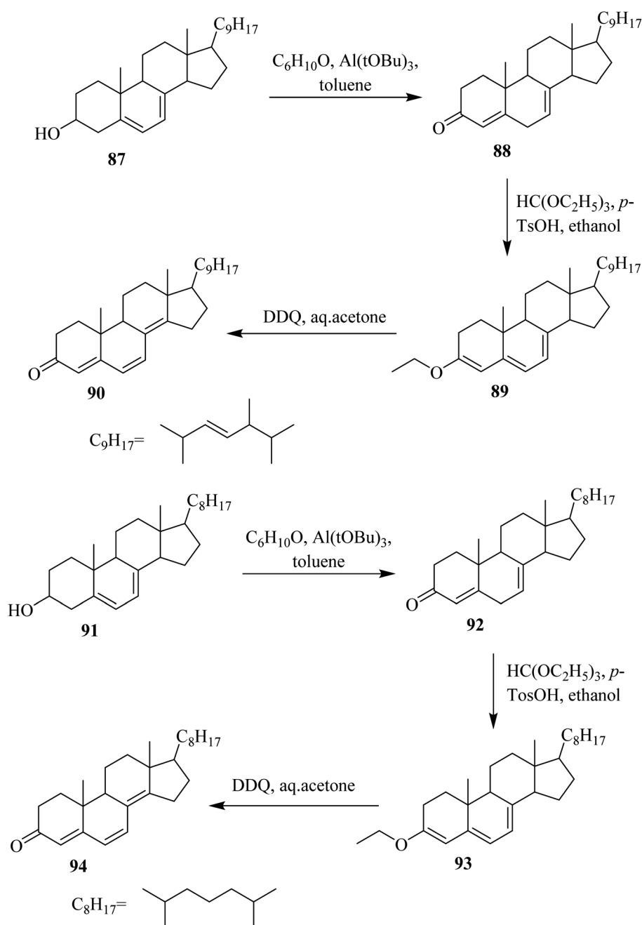
Scheme 38 Synthesis of various steroids structures via DDQ-initiated oxidation.
