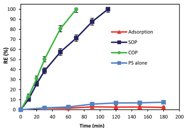
Fig. 6 Contribution of adsorption, SOP, COP and PS alone on cyanide removal (cyanide concentration: 100 mg L -1 , MgO concentration: 500 mg L -1 , ozone concentration: 200 mg h -1 , PS concentration: 200 mg L -1 , pH = 11, reaction time: 180 min).
