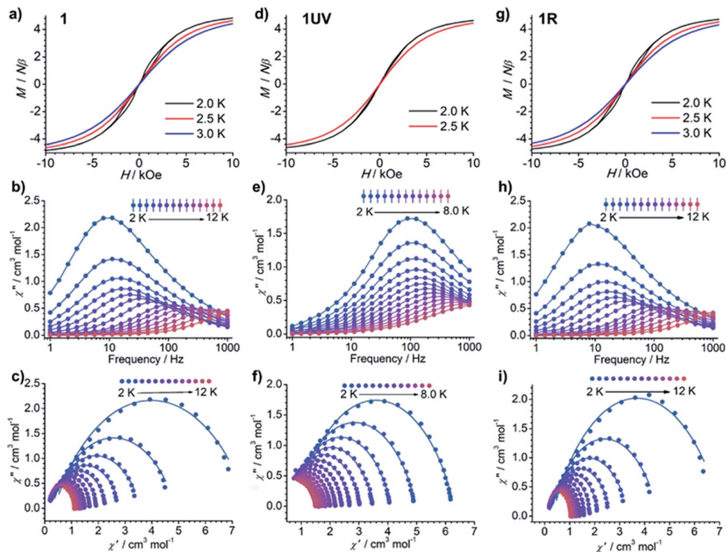
Fig. 9 (a, d and g) The hysteresis curves, (b, e and h) out-of-phase ac susceptibilities ( \chi'' ), and (c, f and i) corresponding Cole–Cole plots for 1 (a–c), 1UV (d–f) and 1R (g–i).
