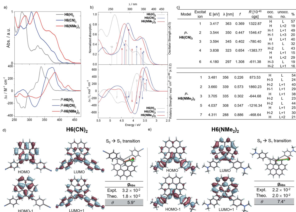
Fig. 5 (a) Top: UV-vis absorption (solid lines) and bottom: ECD spectra of \text{H6(H)}_2 (grey), \text{H6(CN)}_2 (blue) and \text{H6(NMe}_2)_2 (red) in dichloromethane at 298 K ( [\text{c}] \sim 10^{-5} \text{ M} ); (b) calculated (Calc.) absorption (top) and ECD (bottom) of P\text{-H6(H)}_2 (grey), P\text{-H6(CN)}_2 (blue) and P\text{-H6(NMe}_2)_2 (red), selected transitions and oscillator and rotatory strengths indicated as 'stick bars'. (c) Details for the selected transitions and oscillator and rotatory strengths; (d and e) isosurfaces ( \pm 0.04 \text{ au} ) of the frontier molecular orbitals (MOs) with the corresponding electric (green) and magnetic (red) dipole moment vectors corresponding to excitation #2 ( S_0 \rightarrow S_1 transition), and the experimental (Expt.) and calculated (Theo.) absorption dissymmetry factor ( g ) and \theta angle (in degrees) for \text{H6(CN)}_2 and \text{H6(NMe}_2)_2 , respectively.
