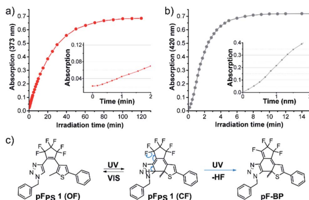
Fig. 8 Kinetic trace of absorption bands formed in \text{pF}_{\text{Ps}} 1 solutions during UV light irradiation (310 nm, 60 \mu\text{M} in (a) methanol (absorption band at 373 nm) and (b) DMSO (absorption band at 420 nm), (c) hypothetical reactions of \text{pF}_{\text{Ps}} 1 in these solvents and the assumed structure of the specific side product \text{pF-BP} .
