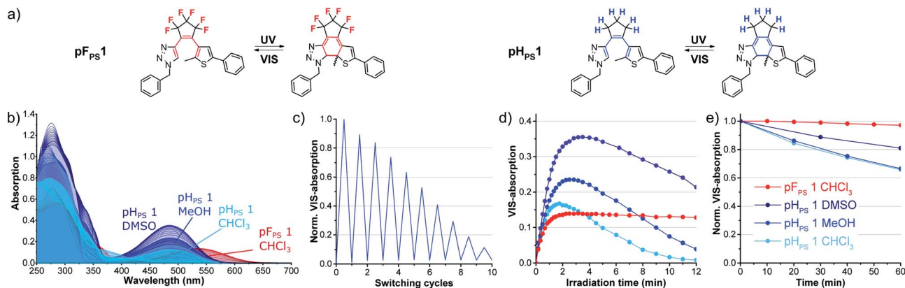
Fig. 7 Comparison of triazole photoswitches with perfluorinated ( \text{pF}_{\text{Ps}} 1 ) and perhydrogenated ( \text{pH}_{\text{Ps}} 1 ) cyclopentene bridge: (a) structures of the respective OF and CF isomers, (b) time-dependent changes in the absorption spectra upon UV light irradiation (310 nm, 60 \mu\text{M} conc.) to the (p)PSS, (c) reversibility of \text{pH}_{\text{Ps}} 1 in methanol, (d) kinetic trace of the VIS absorption bands (CF isomers) during extended UV light irradiation, (e) thermostability (20 ^{\circ}\text{C} ), see also Table S4.†
