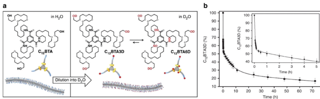
Fig. 3 (a) Chemical structures of C_{12} BTA and its deuterated analogues C_{12} BTA3D and C_{12} BTA6D, schematic representation of the supramolecular polymers formed in water and an illustration of the H/D exchange process. (b) Kinetic profile illustrates hydrogen to deuterium exchange rate of C_{12} BTA3D to C_{12} BTA6D, fit to a triexponential decay. The inset shows an enlargement of the data points and fit for the first 5 h. Adapted from ref. 82, Copyright 2017 Springer Nature.
