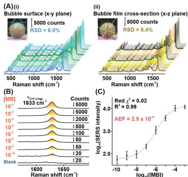
Fig. 3 (A) (i) SERS spectra showing high signal homogeneity across different laser irradiation angles along the (i) bubble surface and (ii) bubble film cross-section. (B) SERS spectra showing the 1633\text{ cm}^{-1} peak changes with varying concentrations of MB. (C) Computing the detection limit and analytical enhancement factor of the Plasmonic bubble using the 1633\text{ cm}^{-1} peak.
