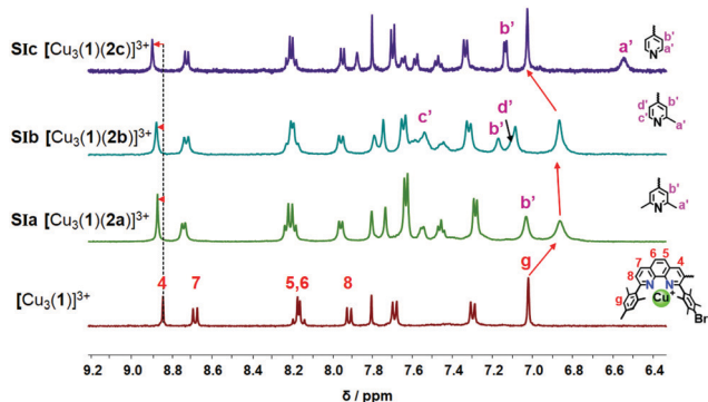
Fig. 2 Comparison of partial ^1\text{H} NMR spectra ( \text{CD}_2\text{Cl}_2 , 500 MHz, 298 K) of copper loaded deck [\text{Cu}_3(\mathbf{1})]^{3+} , SIIa : [\text{Cu}_3(\mathbf{1})(\mathbf{2a})(\mathbf{3})]^{3+} , SIIb : [\text{Cu}_3(\mathbf{1})(\mathbf{2b})(\mathbf{3})]^{3+} , SIIc : [\text{Cu}_3(\mathbf{1})(\mathbf{2c})(\mathbf{3})]^{3+} . For assignment, partial structures of 1 & 2a–c are given.
