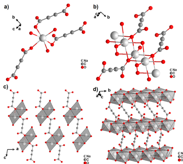
Fig. 5 Crystal structure of hydrated sodium acetylenedicarboxylate [ Na_2(ADC)(H_2O)_4 ] showing: (a) the coordination environment of the Na atom, (b) the coordination mode of ADC linkers and water oxygen atoms, and (c) and (d) sheets from chains of NaO_6 octahedra connected by ADC linkers. Graphics redrawn from the cif file (CSD-Refcode XADSAX). 42
