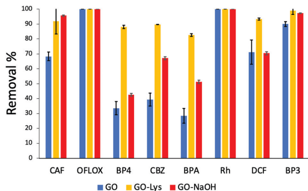
Fig. 2 Removal of EC mix (5 ppm each, V_{\text{tot}} = 25 \text{ mL}^{-1} , 25 mg of sorbent, contact time 24 h (data at 1 h and 4 h are reported in Fig. S7 and S8 ESI ^{\dagger} ). The acronyms refer to the molecules shown in Fig. S1, ESI ^{\dagger} .
