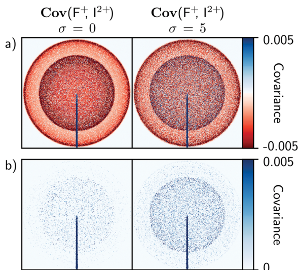
Fig. 5 (a) Recoil-frame covariance images produced from simulated Coulomb explosions of 3,5-difluoriodobenzene into two channels: F^+ and I^+ , or F^+ and I_2^+ . Each image was produced with \nu = 20 and \sigma = 0 or 5. The increase in \sigma produces false correlations between the two channels, which appear as two positive isotropic features at high and low kinetic energies. (b) The positive components of the covariance. Each image is normalized to its maximum value.
