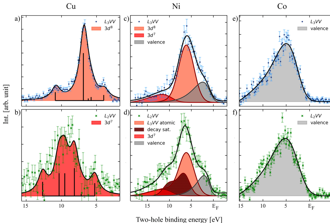
Fig. 1 L_{3VV} (upper panel) and L_{2L3V} (lower panel) CK Auger spectra of Cu (a and b), Ni (c and d) and Co (e and f) recorded in coincidence with the p_{3/2} and the p_{1/2} photoelectrons, respectively. The lifetime broadened atomic multiplet contribution to the spectra is shown in different red tones corresponding to different final states. In grey the itinerant part of the spectra is represented by the self-convolution of the valence band photoelectron spectrum.
