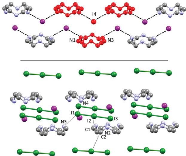
Fig. 3 Top: Visualization of H-bonded (\text{H}_2\text{Cyclen-I})_n^{4+} polycationic ribbons, repeating unit (red), as discussed in Fig. 2. Bottom: Their interaction with \text{I}_3^- counteranions surrounding and spacing such ribbons.
