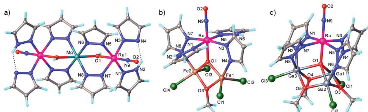
Fig. 10 The structures of (a) [\{\text{Ru}(\mu\text{-OH})(\mu\text{-p-z})_2(\text{p-z})(\text{NO})(\text{Hpz})_2\}_2\text{Mg}] , (b) [\text{Fe}_2\text{RuCl}_4(\mu_3\text{-O})(\mu\text{-OMe})(\mu\text{-p-z})_2(\text{NO})(\text{Hpz})_2] and (c) [\text{Ga}_3\text{RuCl}_3(\mu_4\text{-O})(\mu\text{-OMe})_3(\mu\text{-p-z})_4(\text{NO})] . The structures are taken from those reported on the CSD; codes: (a) LAWGUP, (b) LAWHOK, (c) LAWHIE.
