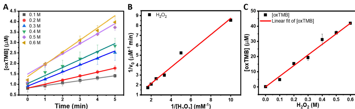
Fig. 5 (A) Temporal evolution of oxTMB concentrations in 0–5 min of the reactions catalyzed by Au@AgAu NRs with different concentrations of H 2 O 2 and (B) Lineweaver–Burk plots for H 2 O 2 . The pH of the reaction solutions was kept at 4.5, and the concentrations of NRs and TMB were 1.6 \times 10^{-10} NPs mL -1 and 750 \mu\text{M} , respectively. The concentrations of oxTMB were obtained using the Beer–Lambert law assuming a molar absorption coefficient of 39 000 M -1 cm -1 at 652 nm. The error bars represent the standard deviation of the three independent measurements. (C) Linear fitting of the variation of oxTMB concentration for different concentrations of H 2 O 2 (0.1–0.6 M).
