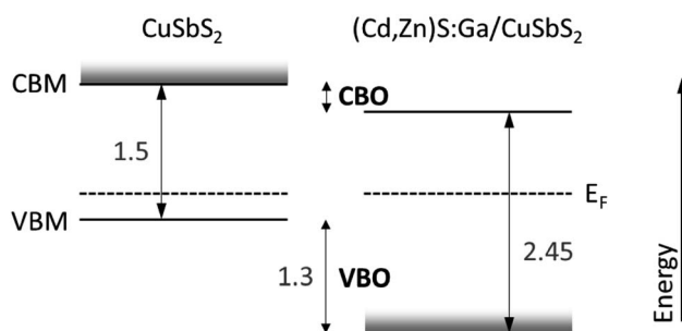
Fig. 8 Schematic presentation of the energy levels at the (Cd,Zn)S:Ga/CuSbS 2 interface. All values are given in eV. The experimentally derived VBO has an uncertainty of \pm 0.1 eV. The band gap values of the buffer and absorber are bulk band gaps from literature. The impact of the chemical interaction at the interface or deviation of the surface from the bulk structure is also depicted as shaded grey areas: the Cu diffusion into the buffer will result in the formation of Cu-derived states close to the buffer VBM (potentially pushing the VBM towards E_F ) and the Cu-deficiency of the CuSbS 2 surface will result in an absorber VBM and CBM shift away from E_F . The first will result in a reduction of the offset in the VB and the latter will lead to an increase of the negative offset in the CB.
