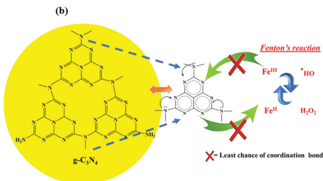
Fig. 8 (a) Alkaline stability of the QPS and QPS-CN x composite membranes in 3 M NaOH for 300 h and (b) the related mechanism showing the stability against Fenton's reagent.
