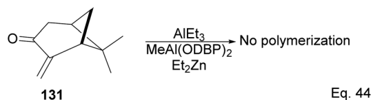
Scheme 38 Lewis acid ( \text{AlEt}_3 )-assisted polymerization of pinacarvone.
