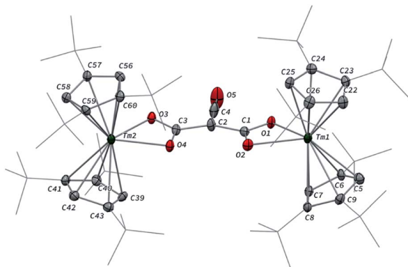
Fig. 6 Molecular structure of 5 in the solid state with thermal ellipsoids at the 40% probability level (except for the t Bu groups depicted in wireframe). H atoms have been omitted for clarity. Selected bond distances (Å) and angles [°]: Tm1–O1 2.282(5), Tm1–O2 2.354(5), Tm2–O3 2.305(5), Tm2–O4 2.318(5), O1–C1 1.283(8), O2–C1 1.263(8), O3–C3 1.273(8), O4–C3 1.267(8), O5–C4 1.142(10), C1–C2 1.460(9), C2–C3 1.461(10), C2–C4 1.343(10); O1–Tm1–O2 56.9(2), O3–Tm2–O4 57.0(2), O1–C1–C2 116.0(6), O2–C1–O1 120.3(6), O2–C1–C2 123.6(6), C1–C2–C3 131.7(6), C1–C2–C4 113.0(7), C3–C2–C4 115.3(6), O3–C3–C2 118.1(6), O3–C3–O4 120.5(6), O4–C3–C2 121.4(6), O5–C4–C2 178.5(10).
