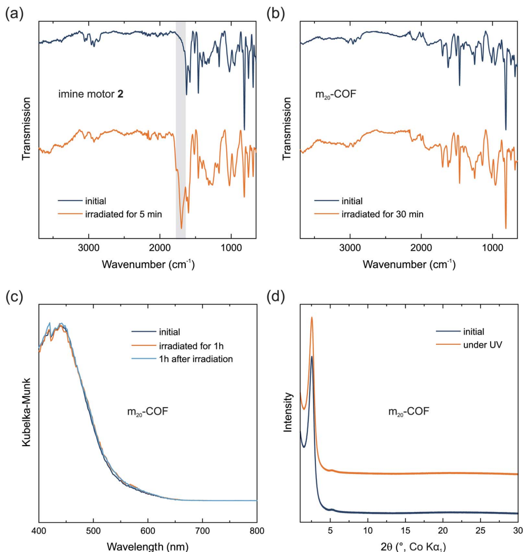
Fig. 5 FT-IR spectra of a thin film of the imine motor 2 (a) and m_{20} -COF (b) under prolonged irradiation at 365 nm (UV-LED). Grey area highlights appearing C=O vibrations during irradiation of imine motor 2. Direct reflectance UV/vis spectra (c) and XRPD patterns (d) of m_{20} -COF before and during irradiation (>1.5 h) at 365 nm are shown. The patterns are stacked with an arbitrary offset to aid visibility.
