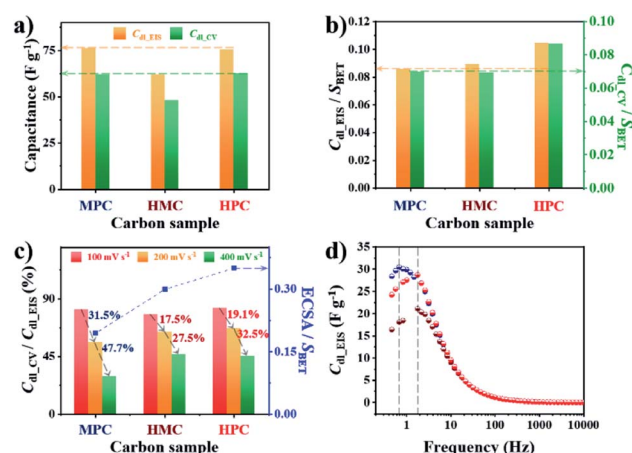
Fig. 2 (a) Electric double layer capacitance calculated from EIS measured at OCP ( C_{\text{dl,EIS}} ) and CV measured at 100\text{ mV s}^{-1} ( C_{\text{dl, CV}} ) of MPC, HMC and HPC. (b) C_{\text{dl,EIS}} and C_{\text{dl, CV}} of MPC, HMC and HPC normalized by their S_{\text{BET}} . (c) The ratio between C_{\text{dl, CV}} and C_{\text{dl,EIS}} at high scan rates (100, 200 and 400\text{ mV s}^{-1} ) and electrochemically active surface area (ECSA) normalized by S_{\text{BET}} of MPC, HMC and HPC. (d) Imaginary part of complex capacitance ( C_{\text{im}} ) at OCP.
