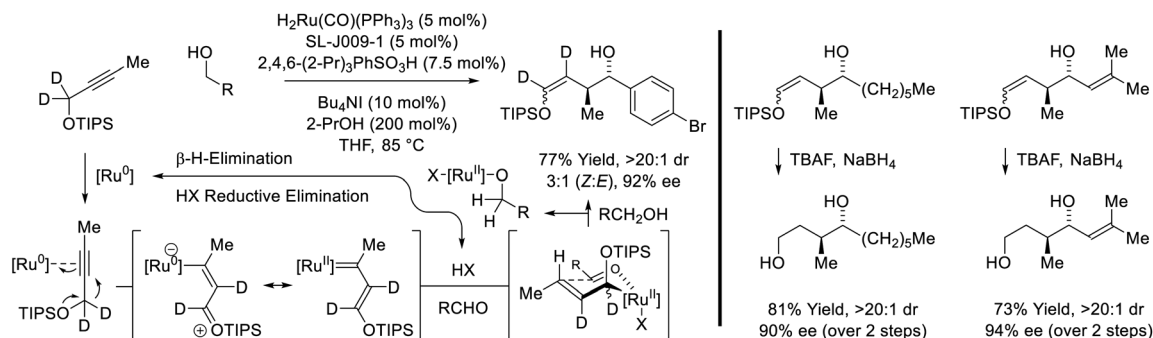
Scheme 9 anti -Diastereo- and enantioselective conversion of primary alcohols and trialkylsilyl propargyl ethers to branched secondary alcohols.
