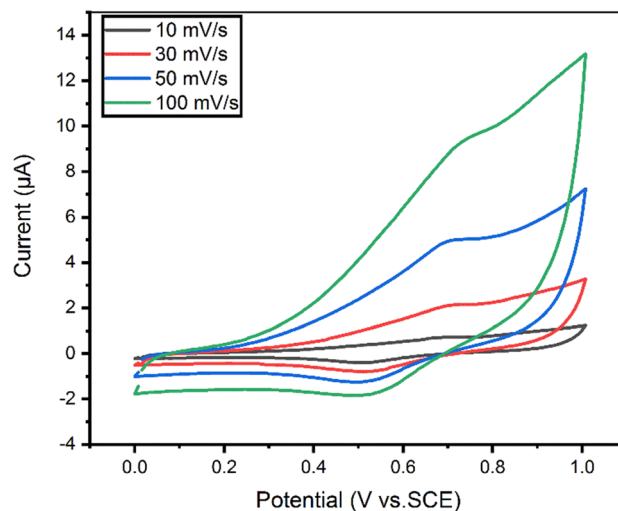
Fig. 3 Effect of CV scan rate on 100 \mu M 5-CP in 0.1 M PBS for the rGO/MOF/AuE. The scan rate was varied to be 10, 30, 50, and 100 mV s -1 .
