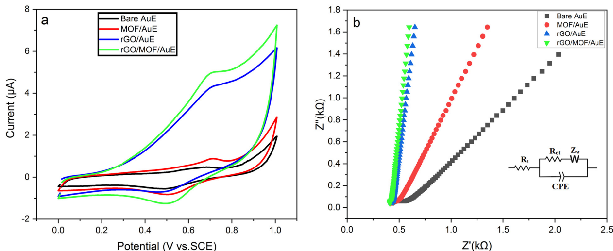
Fig. 2 (a) CVs of 5 mM 5-CP at different modified gold electrodes (AuEs) in the 0.1 M PBS at a scan rate of 50 mV s -1 . (b) EIS between 10 -1 and 10 5 Hz, the experiment solution is 0.1 M PBS pH = 7.0 containing [Fe(CN) 6 ] 3-/4- .
