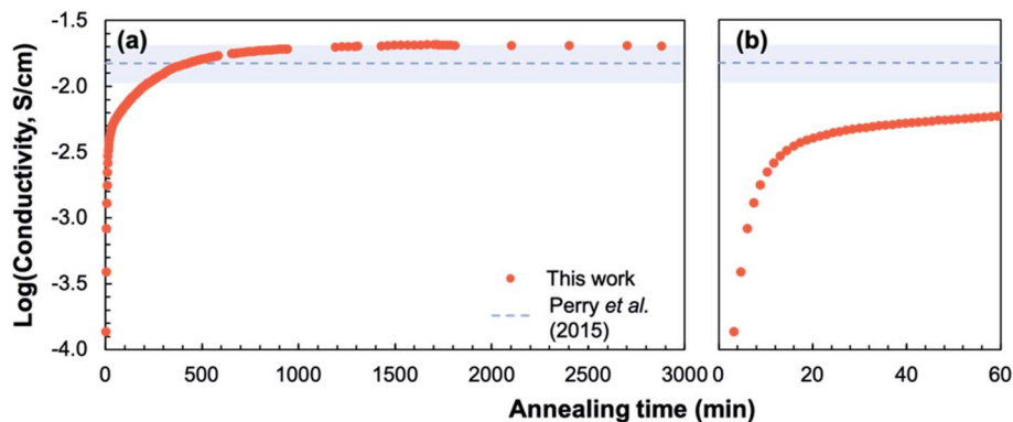
Fig. 10 Plot of conductivity over the full annealing period (a) and over the first hour (b) at 400 °C in ~0.2 atm UHP O 2 and ~0.8 atm UHP Ar; dashed line shows the conductivity and conservative uncertainty estimate (shaded blue) of a crystalline-grown STF35 thin film 26 under the same conditions.
