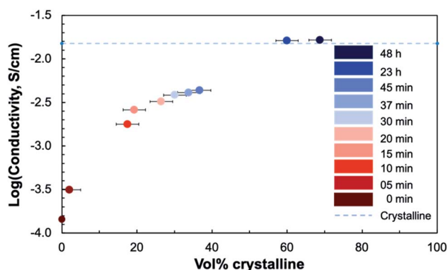
Fig. 11 Plot of the logarithmic in-plane total conductivity at 400 °C in ~0.2 atm UHP O 2 and ~0.8 atm UHP Ar as a function of crystalline volume percent of crystallizing STF35 thin films. The conductivity of a crystalline-grown STF35 thin film, from ref. 26, measured under the same conditions is marked by the dashed line.
