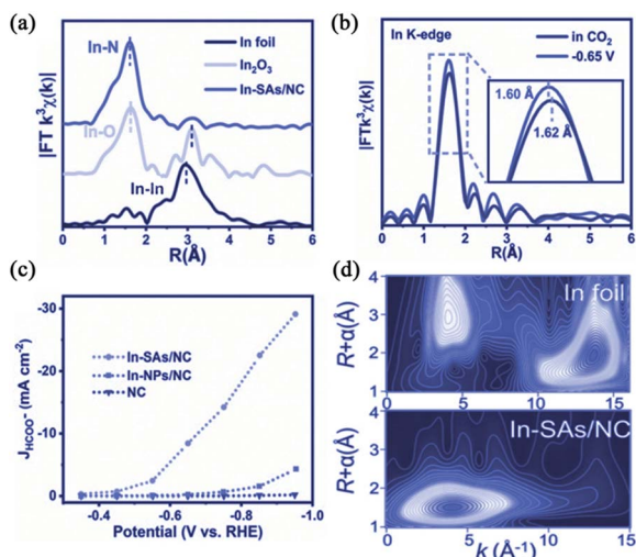
Fig. 8 (a) In K-edge spectra of In-SAs/NC, In 2 O 3 and In foil; (b) in situ spectra of In-SAs/NC; (c) the current density of HCOO - in CO 2 RR; (d) WT-EXAFS spectrums. Reprinted with permission from ref. 114. Copyright 2020, WILEY-VCH GmbH.
