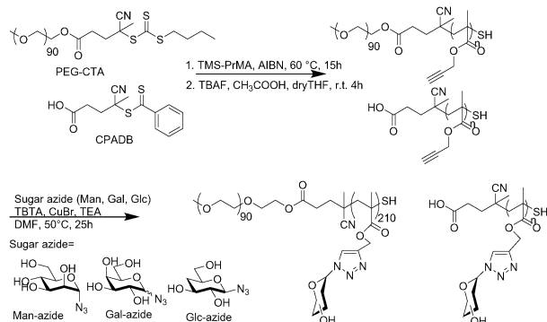
Scheme 1 Preparation of glycopolymers in this study via RAFT polymerization and the Huisgen reaction.
