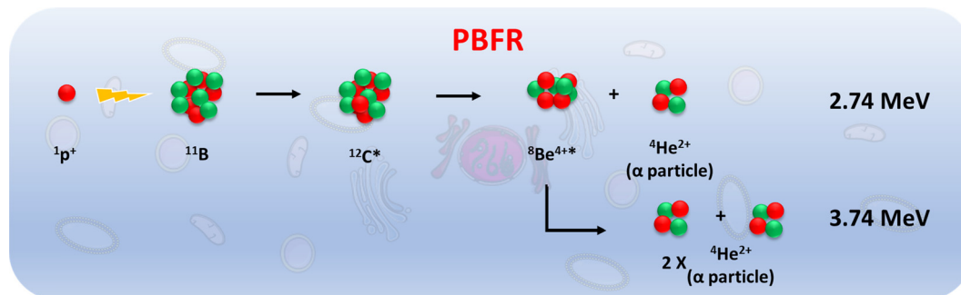
Scheme 2 Representation of the reaction between an energetic proton and ^{11}\text{B} resulting in the generation of excited carbon ^{12}\text{C} , which splits into a 2.74 MeV \alpha particle and a ^8\text{Be} . Then, beryllium divides into two \alpha particles. Consequently, a total of three \alpha particles are generated by the proton boron reaction.
