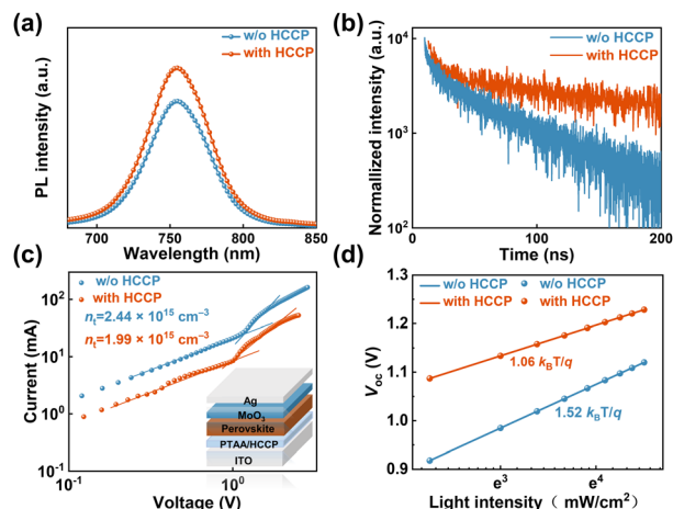
Fig. 3 (a) Steady-state and (b) time-resolved PL spectra. (c) Dark I – V curves of the hole-only device (illustrated as a single-hole device structure) (d) Light intensity-dependent open-circuit voltage measurements.
