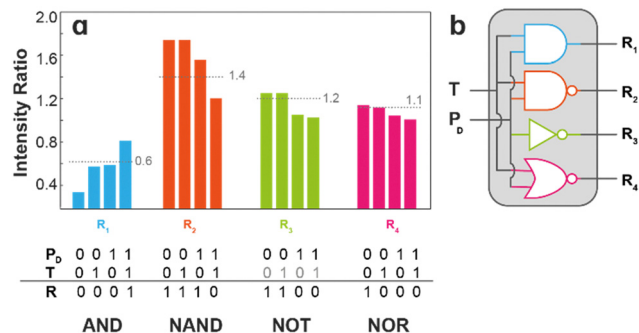
Fig. 11 (a) Bar chart of the intensity ratios R_1 – R_4 as a function of the temperature input ( T ) and excitation power density ( P_D ) presenting the corresponding threshold (pointed line) the truth tables in the bottom. (b) Schematic representation of the logic circuitry with the logic gates presented in (a). Figure reproduced from ref. 81.
