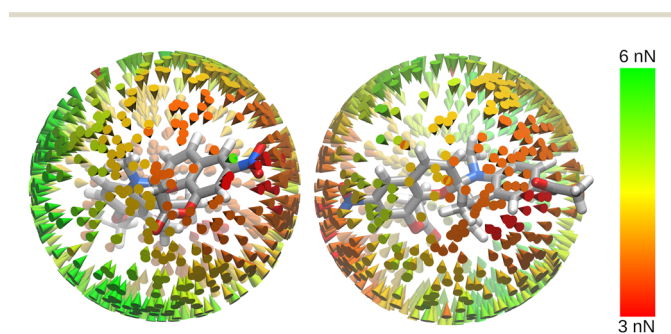
Fig. 5 Rupture forces of B with an electric field (0.01 a.u.) applied at different, randomly chosen angles, calculated with EFEI. The structure is shown from two opposing sides. Fields applied in the direction of red cones lead to lower rupture forces, green cones indicate directions along which rupture forces remain higher.
