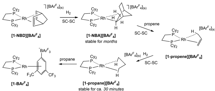
Scheme 1 Synthesis of \sigma -alkane complexes via single crystal-to-single crystal (SC–SC) transformations: (a) [\mathbf{1-NBA}][\text{BAR}^F_4] by hydrogenation of [\mathbf{1-NBD}][\text{BAR}^F_4] ; (b) [\mathbf{1-propane}][\text{BAR}^F_4] from [\mathbf{1-NBA}][\text{BAR}^F_4] via sequential NBA/propene substitution and hydrogenation.
