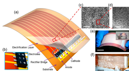
Fig. 7 Structure of a thin-film triboelectric generator (TF-TEG). a, Schematic diagram of an arrayed TF-TEG. b, Enlarged sketch of the arrayed bridge rectifiers. c, SEM image of the PTFE nanoparticles on the electrification layer (scale bar = 1 μm). d, Enlarged view of the nanoparticles at a tilted angle of 60° (scale bar = 500 nm). e, Picture of a bendable as-fabricated TF-TEG. Inset: Water contact angle on the nanostructured surface (scale bar = 25 mm). f, Picture of the TF-TEG that is interacting with the water wave (scale bar = 25 mm) (figures and captions reproduced from ref. 33 with permission from American Chemical Society, copyright 2015).
