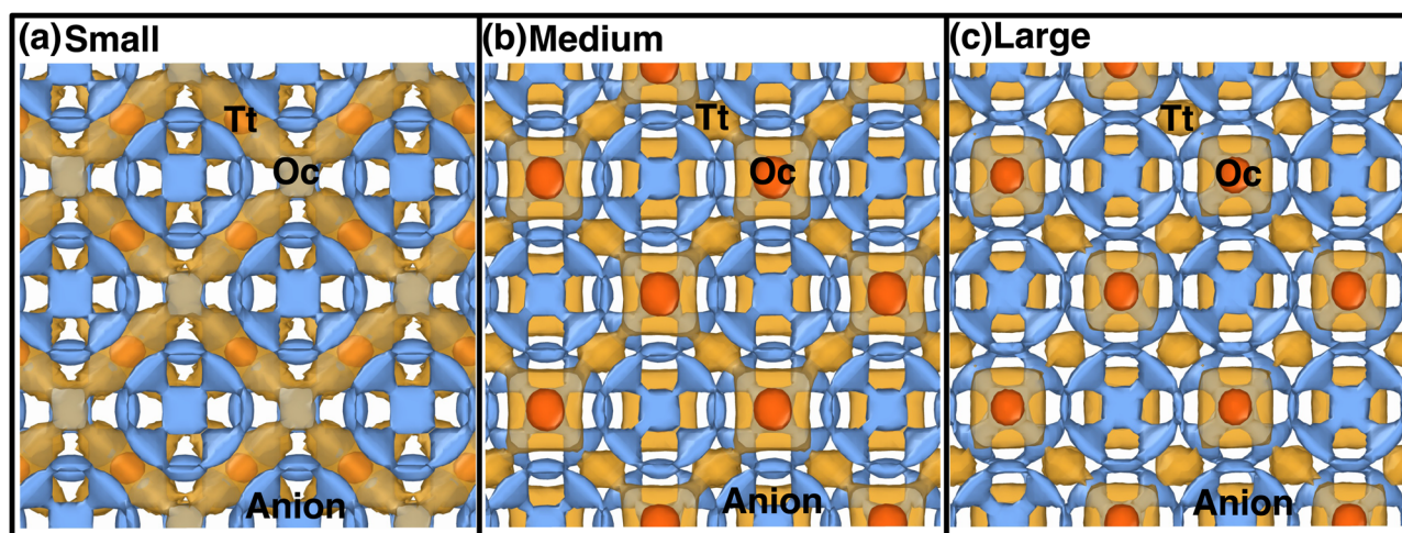
Fig. 8 Isosurface density plots of the cation (isovalues of 2 \times 10^{-4} \text{ \AA}^{-3} (orange) and 6 \times 10^{-5} \text{ \AA}^{-3} (red)) and H-atom for \text{MCB}_{11}\text{H}_{12} ( M = small, medium, and large) in a 2 \times 2 \times 2 supercell obtained using OVITO 70 software at 475 K from NVE-MD simulations. (a) Isovalue 7.5 \times 10^{-5} \text{ \AA}^{-3} (blue) for small-sized cation. (b) Isovalue 7.5 \times 10^{-5} \text{ \AA}^{-3} (blue) for medium-sized cation. (c) Isovalue 7.5 \times 10^{-5} \text{ \AA}^{-3} (blue) for large-sized cation. Tt- and Oc-sites formed by anions are marked. We choose different H isovalues for different sizes of cation cases for better visualization.
