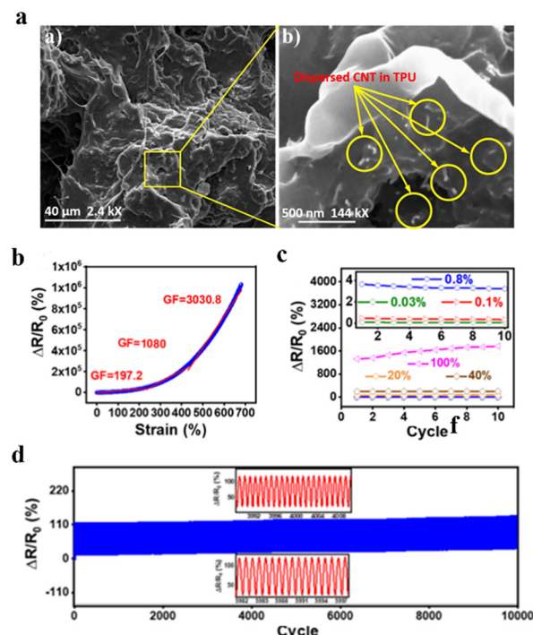
Fig. 12 (a) SEM images of TPU/MWCNTs/AgNPs. Reproduced with permission from ref. 180. Copyright 2019, Wiley-VCH. (b) \Delta R/R_0 of CPUF vs strain. (c) Maximum values of CPUF at the strain of 0.03% to 100%. (d) Long-term stability during 10 000 cycles. Reproduced with permission from ref. 182. Copyright 2022, the American Chemistry Society.
