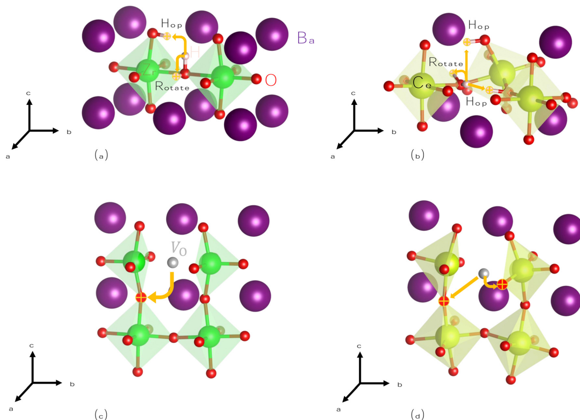
Fig. 4 Hopping and rotation migration pathways for hydrogen and oxygen diffusion in BaZrO 3 and BaCeO 3 . Migration pathways of interstitial protons ( \text{H}_{\text{i}}^{+} ) in (a) bulk BaZrO 3 and (b) bulk BaCeO 3 , and hopping migration pathways of oxygen vacancies ( \text{V}_{\text{O}}^{2+} ) in (c) bulk BaZrO 3 and (d) bulk BaCeO 3 .
