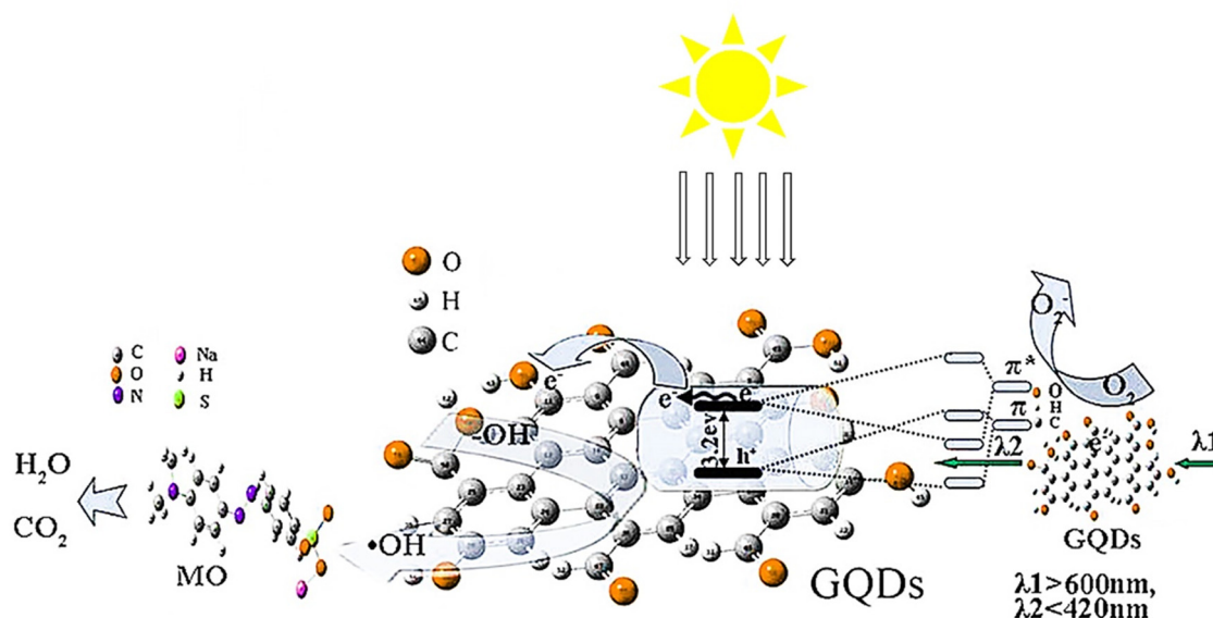
Fig. 13 The schematic of the improved light-driven photocatalysis of \text{GQD}/\text{TiO}_2 -NT composites. Reproduced with permission from ref. 110. Copyright (2016) Elsevier.
