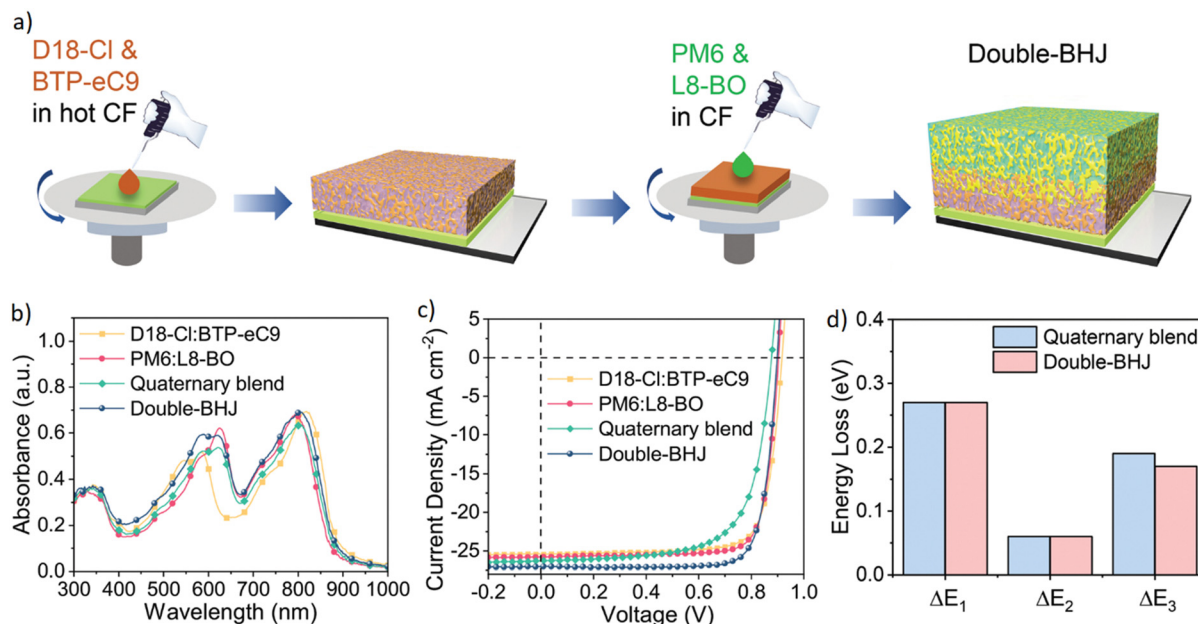
Fig. 13 (a) Schematic representation of the multicomponent OSCs prepared by sequential deposition. (b) Absorption spectra of the active layers. (c) Corresponding J - V curves. (d) Energy loss in the devices. Reprinted with permission from ref. 72. Copyright 2023, Wiley-VCH.
