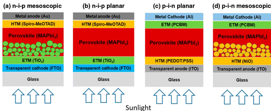
Fig. 4 Diagram displaying the four-layered assemblies of PSCs (a) n-i-p mesoscopic, (b) n-i-p planar, (c) p-i-n planar, and (d) p-i-n meso-structured (reproduced with permission from ref. 36, copyright 2016 SPIE).
