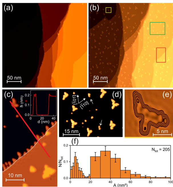
Fig. 1 Cluster formation through laser illumination: (a) and (b) large-scale images (a) before and (b) after illumination at 7.6 \text{ mJ cm}^{-2} absorbed fluence, 400 \text{ nm} , 50 \text{ fs} , 10^7 pulses; red rectangle marks region with a step, enlarged in panel (c); green rectangle marks a terrace region, enlarged in panel (d); yellow rectangle marks a dendritic island, enlarged in panel (e); a dotted white line in (c) marks the position of the original step edge as extracted from the image before illumination. Inset: Height profile along the red line in the STM image. Arrows in (d) mark the onset of the agglomeration of small clusters (see text); surface directions of Cu(111) are inferred from images with atomic resolution. A cyclic scale is used in (e) to emphasize the details on top of the cluster. (f) island area histogram of the panel (b) at a bin size of 2 \text{ nm}^2 and 10 \text{ nm}^2 for island areas < 20 \text{ nm}^2 and > 20 \text{ nm}^2 , respectively.
