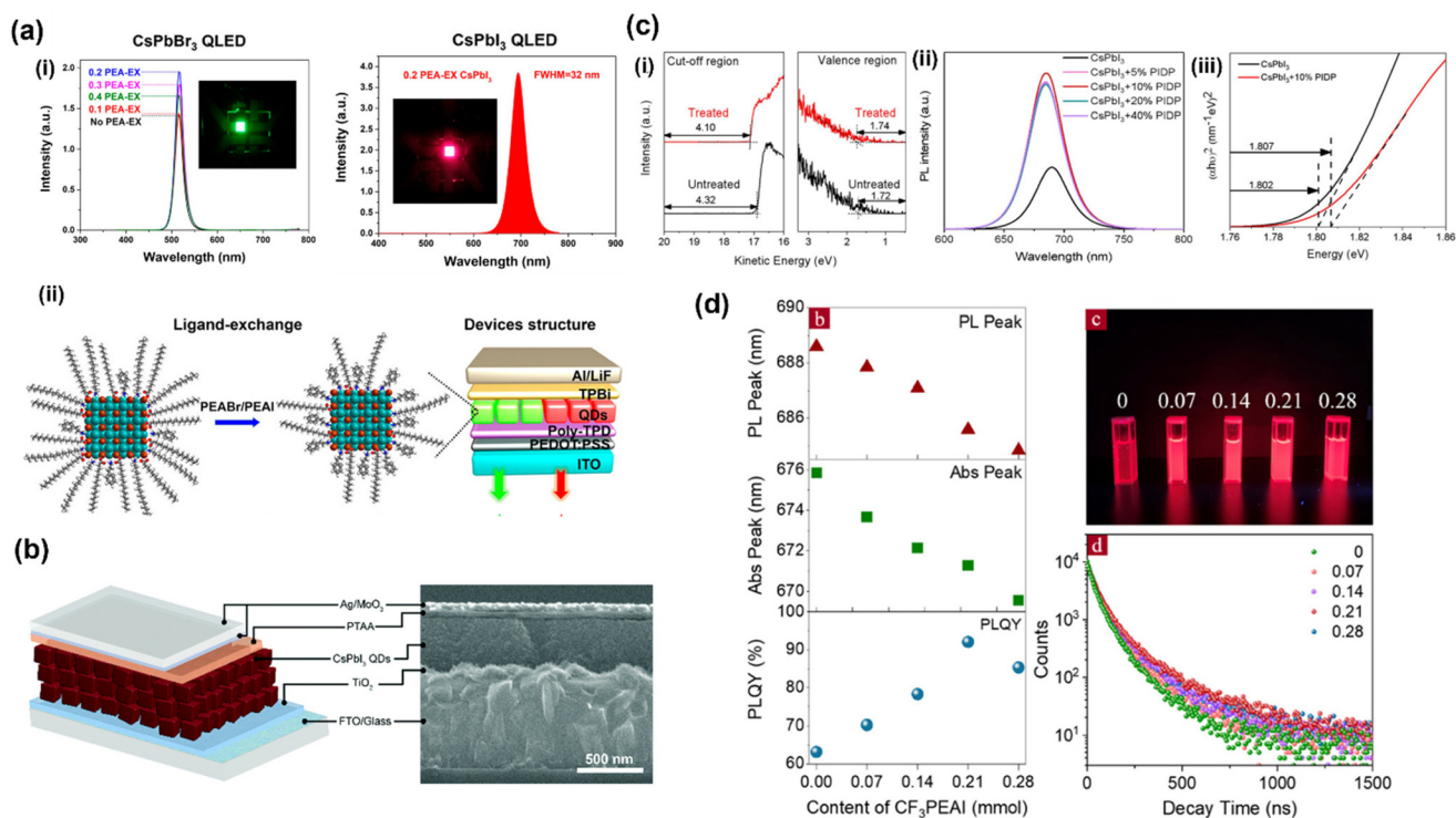
Fig. 4 Selected examples of halogenated AA-HPNC studies. (a) Schematic of the ligand exchange to partially replace OA with PEA Br /PEAI for the fabrication of high-performance CsPbBr 3 and CsPbI 3 QLEDs and the corresponding photographs and emission spectra of the QLEDs. 89 (b) PL lifetimes of CsPbI 3 HPNCs at different PEA concentrations together with the diagram and SEM image of the corresponding fabricated solar cells. 88 (c) (i) PL spectra of CsPbI 3 NCs as a function of PEA concentrations under 405 nm light. (ii) Impact of treatment time on PLQY of the pristine and the PIDP-treated CsPbI 3 NCs. (iii) UPS spectra and Tauc plots of pristine and PIDP-treated CsPbI 3 NCs. 90 (d) The effect of different amounts of CF 3 PEAI on the optical properties CsPbI 3 NCs. 91 Reproduced and/or modified with permissions from the listed references. Panel 4a and d adapted with permission from ref. 89 and 91 Copyright 2018, 2022 American Chemical Society.
