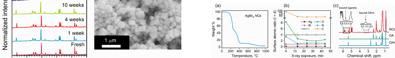
Fig. 6 (a) TGA data for a AgBiI 4 NC sample. (b) Changes in surface composition (atomic ratios normalized to I = 4) of AgBiI 4 film sample during XPS measurement of five consecutive cycles of spectra (Bi 4f → I 3d → Ag 3d → O 1s → C 1s → N 1s, duration of a cycle ~10 min). (c) 1 H NMR spectra of AgBiI 4 NCs, pure OA, and pure OlAm. The insets highlight the proton resonances related to bound ligands.
