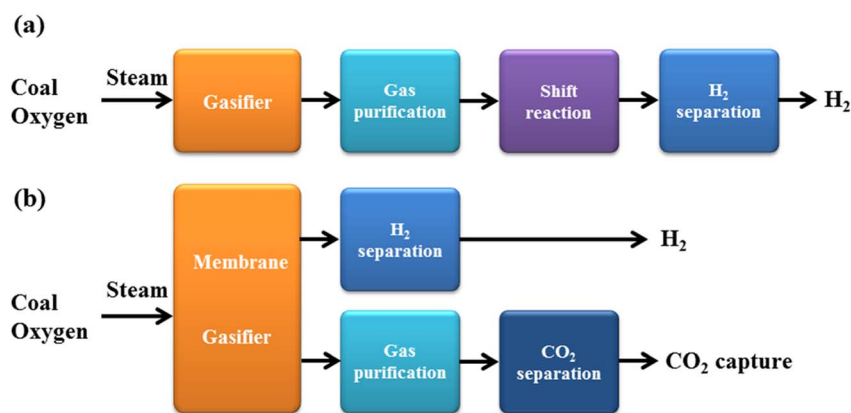
Fig. 9 General schematic for hydrogen production from: (a) traditional process of coal gasification, (b) modified process of coal membrane gasification with CO 2 capture.
