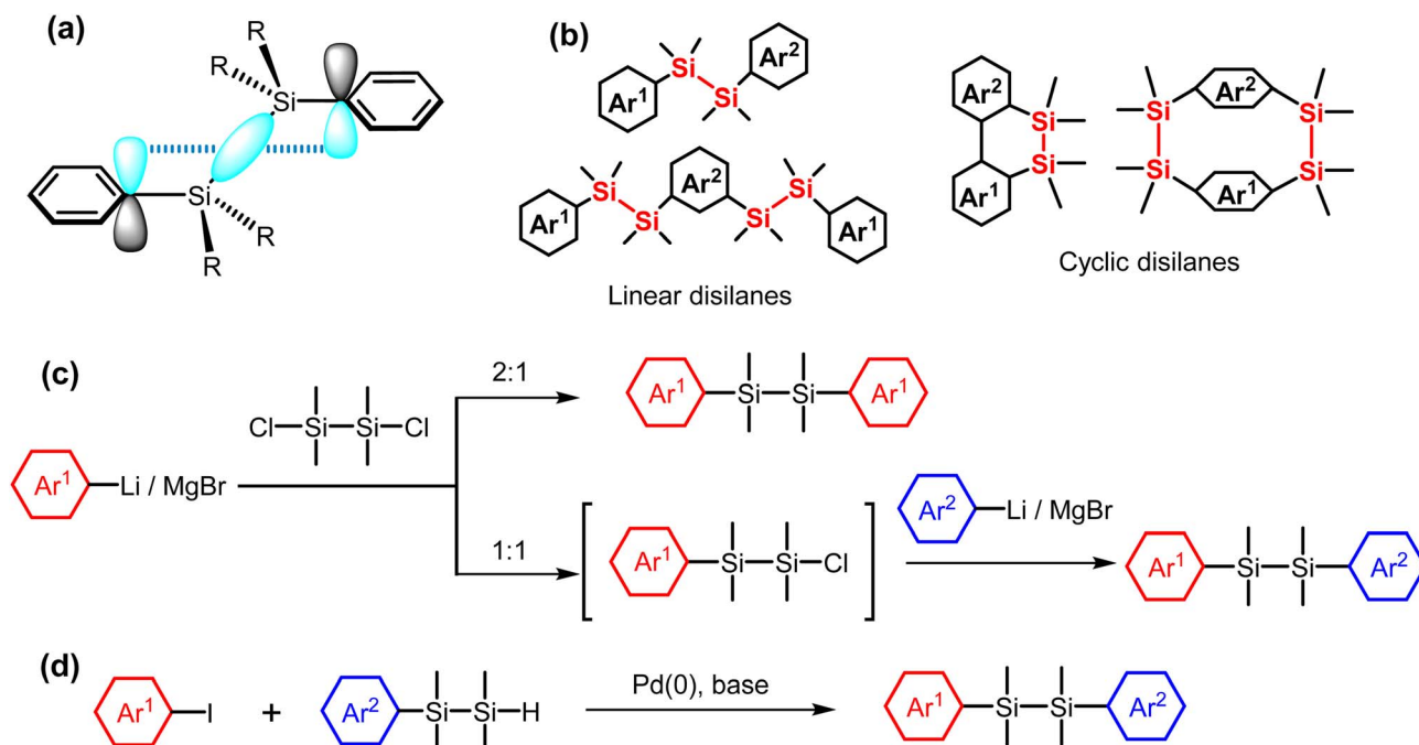
Fig. 1 (a) Schematic representation of \sigma - \pi conjugation in aryl-disilane. (b) The scope of this review. (c) Salt elimination reaction to synthesize disilane-bridged architectures. (d) Pd-catalyzed cross-coupling reaction.
