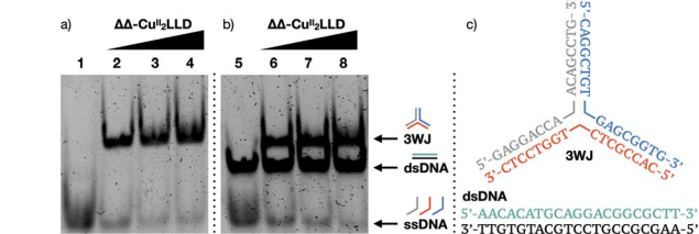
Fig. 3 (a) 10% native PAGE analysis of 3WJ strands in the absence (lane 1) and presence 1, 2 and 3 equivalents of \Delta\Delta -Cu II 2 L L \Delta (lanes 2–4); (b) 3WJ strands and dsDNA in the absence (lane 5) and presence of \Delta\Delta -Cu II 2 L L \Delta (1–3 eq. in lanes 6–8, respectively). 3WJ remains as single-stranded DNA in the absence of \Delta\Delta -Cu II 2 L L \Delta and forms the 3WJ when \Delta\Delta -Cu II 2 L L \Delta is present. In contrast, dsDNA can be visualised in lanes 5–8 and remains unchanged in the presence of increasing concentrations of the Cu II peptide helicate, demonstrating the low affinity of the metalloprotein for canonical DNA; (c) 3WJ and dsDNA sequences used for PAGE analysis.
