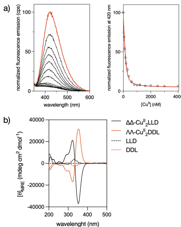
Fig. 1 (a) (Left) Normalized emission spectrum of a 200 nM solution of LLD in phosphate buffer (1 mM, NaCl 10 mM, pH 7.0, orange line), and spectra of the same solution in the presence of increasing concentrations of Cu II ions (black lines). (Right) Titration profile of three independent fluorometric titration experiments at 420 nm and best fit according to the 1 : 2 model in DynaFit (same range as main plot). \lambda_{\text{exc}} = 308 nm. (b) CD spectra of 5 \mu\text{M} solutions of LLD (black dashed line) and DDL (orange dashed line) ligands in phosphate buffer (1 mM, 10 mM NaCl, pH 7.0), and in the presence of 25 \mu\text{M} Cu II ions (same colours, continuous lines).
