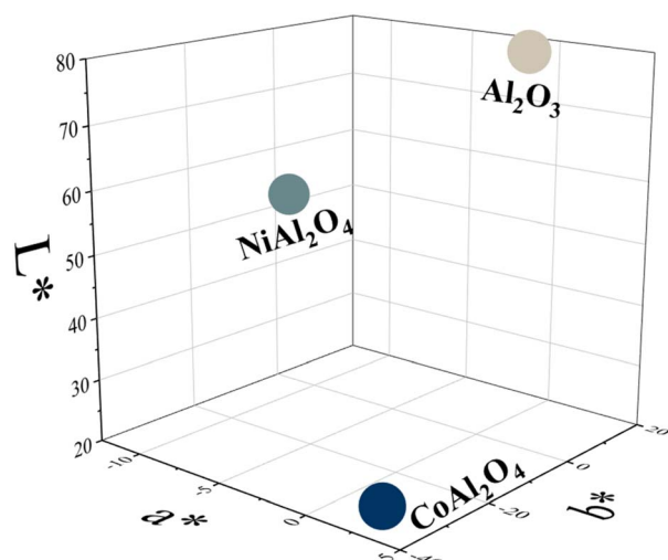
Fig. 9 Distribution of Al 2 O 3 (alumina), CoAl 2 O 4 (cobalt aluminate), and NiAl 2 O 4 (nickel aluminate) in 3D CIE L*a*b* color space.
