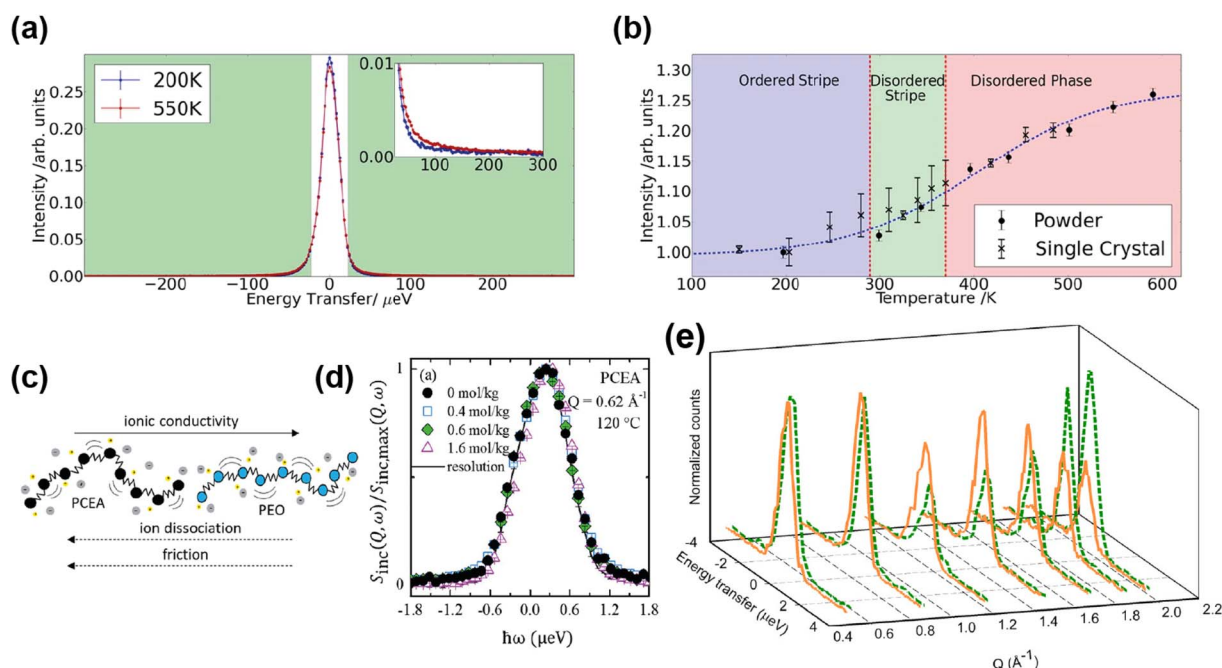
Fig. 23 (a) QENS spectra from \text{Na}_{0.8}\text{CoO}_2 at T 200 K (blue) and T 550 K (red) integrated over Q . Inset shows increase in the quasi-elastic region. (b) QENS intensity integrated over Q and energy transfer as a function of temperature for the powder and single-crystal samples of \text{Na}_{0.8}\text{CoO}_2 . 101 Copyright 2018, CC BY 4.0. (c) Representation of PEO and PCEA polymers. (d) Normalized incoherent structure factor, S_{\text{inc}}(Q, \omega)/S_{\text{inc,max}}(Q, \omega) , in the frequency domain, plotted as a function of energy, h\omega , at Q = 0.62 \text{ \AA}^{-1} and 120 °C. Reprinted with permission from ref. 103 Copyright (2020) American Chemical Society. (e) QENS spectra recorded for ^7\text{Li}(\text{BD}_4)_{0.75}\text{I}_{0.25} at 300 K, without (orange solid line) and with (green dashed line) the application of a potential ( f = 1 \text{ kHz} , U = 3 \text{ V} , and I = 0.4 \text{ mA} ). 107 Reprinted with permission from ref. 107 Copyright 2013 American Chemical Society.
