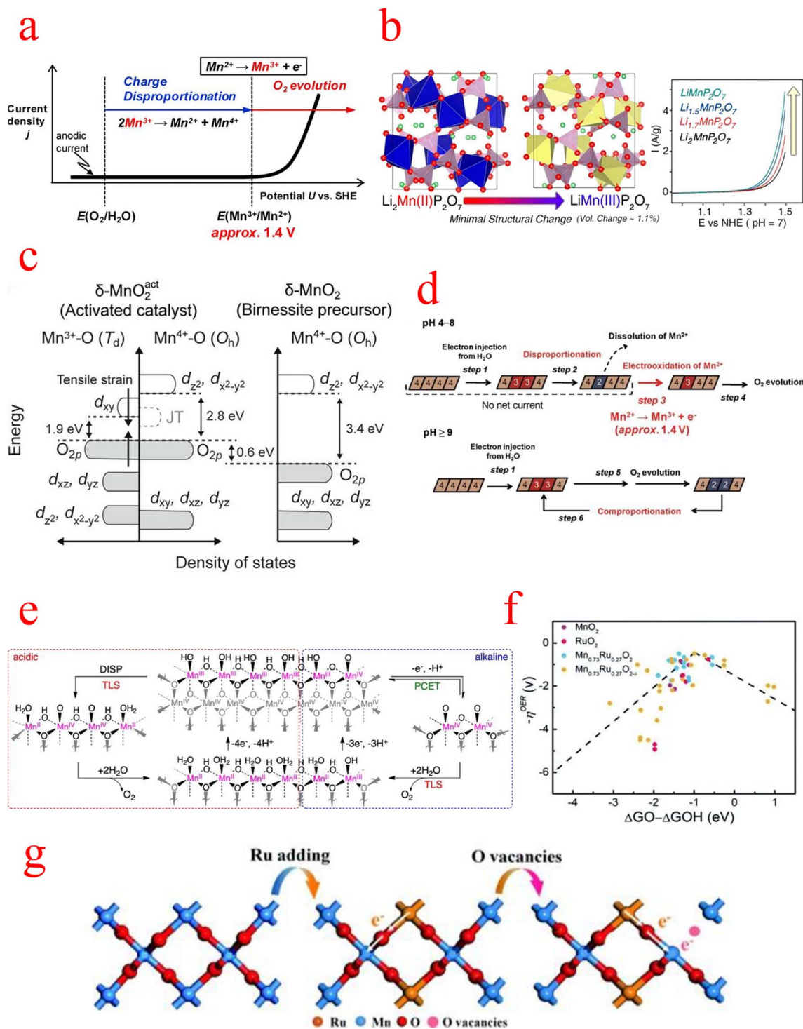
Fig. 7 (a) Schematic illustration of a current density ( j ) vs. potential ( U ) curve for a pristine \delta - MnO_2 electrode under neutral pH conditions. (b) Increase in the average oxidation state of Mn from 2 to 3 in Li_{2-x}MnP_2O_7 and schematic representation of the catalytic performance. (c) Schematic diagram of the band structure of the activated catalyst system derived from the " \alpha - Mn_3O_4-3e^- " model. (d) Schematic diagram of the oxidation state of Mn ions in the \delta - MnO_2 reaction at different pH values. (e) Proposed mechanism for the OER on MnO_x under (left) acidic and (right) alkaline pH conditions. (f) Schematic free energy profiles of overpotential results versus the difference between the adsorption energies of O^* and OH^* intermediates for MnO_2 , etc. in acid media. (g) A schematic diagram of the charge redistribution process in Mn_{0.73}Ru_{0.27}O_{2-\delta} . (a) Reproduced with permission from ref. 101. Copyright 2012, American Chemical Society. (b) Reproduced with permission from ref. 102. Copyright 2014, American Chemical Society. (c) Reproduced with permission from ref. 105. Copyright 2018, Proceedings of the National Academy of Sciences of the United States of America. (d) Reproduced with permission from ref. 107. Copyright 2012, American Chemical Society. (e) Reproduced with permission from ref. 108. Copyright 2014, American Chemical Society. (f and g) Reproduced with permission from ref. 109. Copyright 2022, RSC Publishing.
