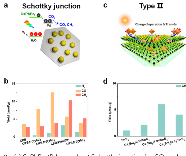
Fig. 9 (a) CsPbBr 3 /Pd nanosheet Schottky junction for CO 2 reduction; reproduced from ref. 98 with permission from American Chemical Society, copyright 2018. (b) Photocatalytic CO 2 reduction performances after 3 h of constant illumination; 100, 300, 600, and 900 mean the volume ( \mu\text{L} ) of added Pd nanosheets; CsPbBr 3 : abbreviated as CPB; reproduced from ref. 98 with permission from American Chemical Society, copyright 2018. (c) Cs 2 SnI 6 /SnS 2 nanosheet type-II heterojunction for CO 2 reduction; reproduced from ref. 106 with permission from American Chemical Society, copyright 2010. (d) Photocatalytic CO 2 reduction to CH 4 of SnS 2 , Cs 2 SnI 6 (0.5)/SnS 2 , Cs 2 SnI 6 (1.0)/SnS 2 , and Cs 2 SnI 6 (2.0)/SnS 2 nanocomposites; 0.5, 1.0, and 2.0 correspond to the concentration (1.0 mM, 2.0 mM, and 4.0 mM) of CsI; reproduced from ref. 106 with permission from American Chemical Society, copyright 2019.
