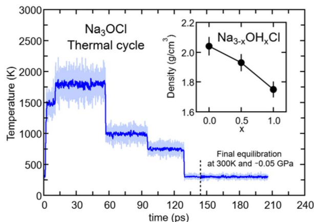
Fig. 1 (Color online) Temperatures along the thermal cycle for amorphous \text{Na}_3\text{OCl} : light blue line, instantaneous T values; blue line, T value sliding average with a window of 0.1 ps. The dashed vertical grey line sets the time at which the optimization of the volume at T = 300 K and 0 GPa was implemented. Inset: final density values optimized at T = 300 K for the three \text{Na}_{3-x}\text{OH}_x\text{Cl} models. Error bars are estimated with tests at different volumes performed on several final configurations (300 K) to obtain a final stress tensor close to 0 GPa (see Fig. S1 in the ESI†).
